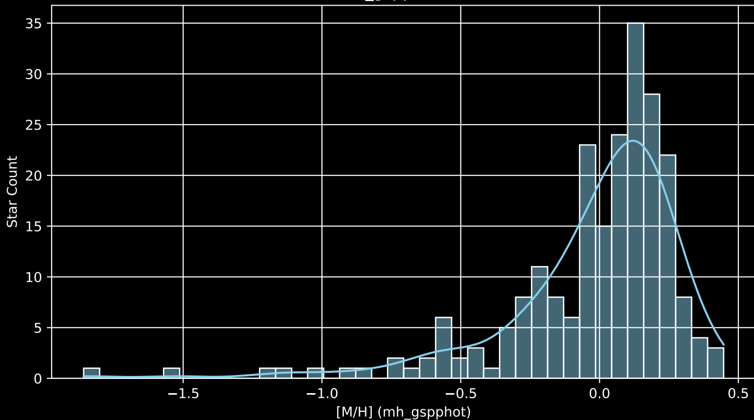
APOGEE DR17 Field: [020-06 [M/H] (mh_gspphot) (n= 224)
