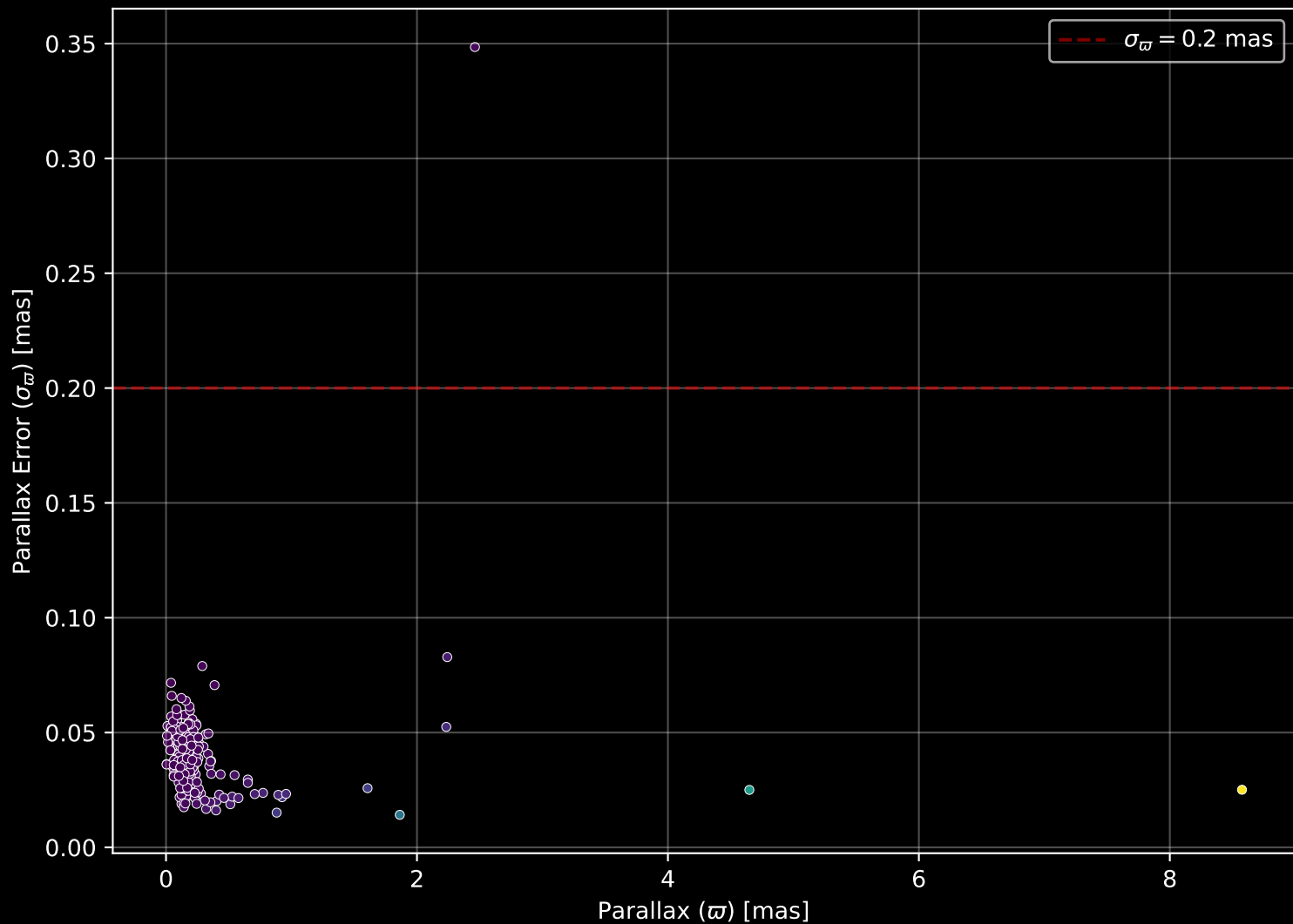
APOGEE DR17 Field: [020-06] Parallax Quality (n= 225)
