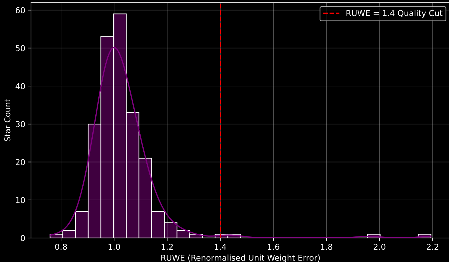
GAPOGEE DR17 Field [020-06] RUWE Distribution (n= 224)
