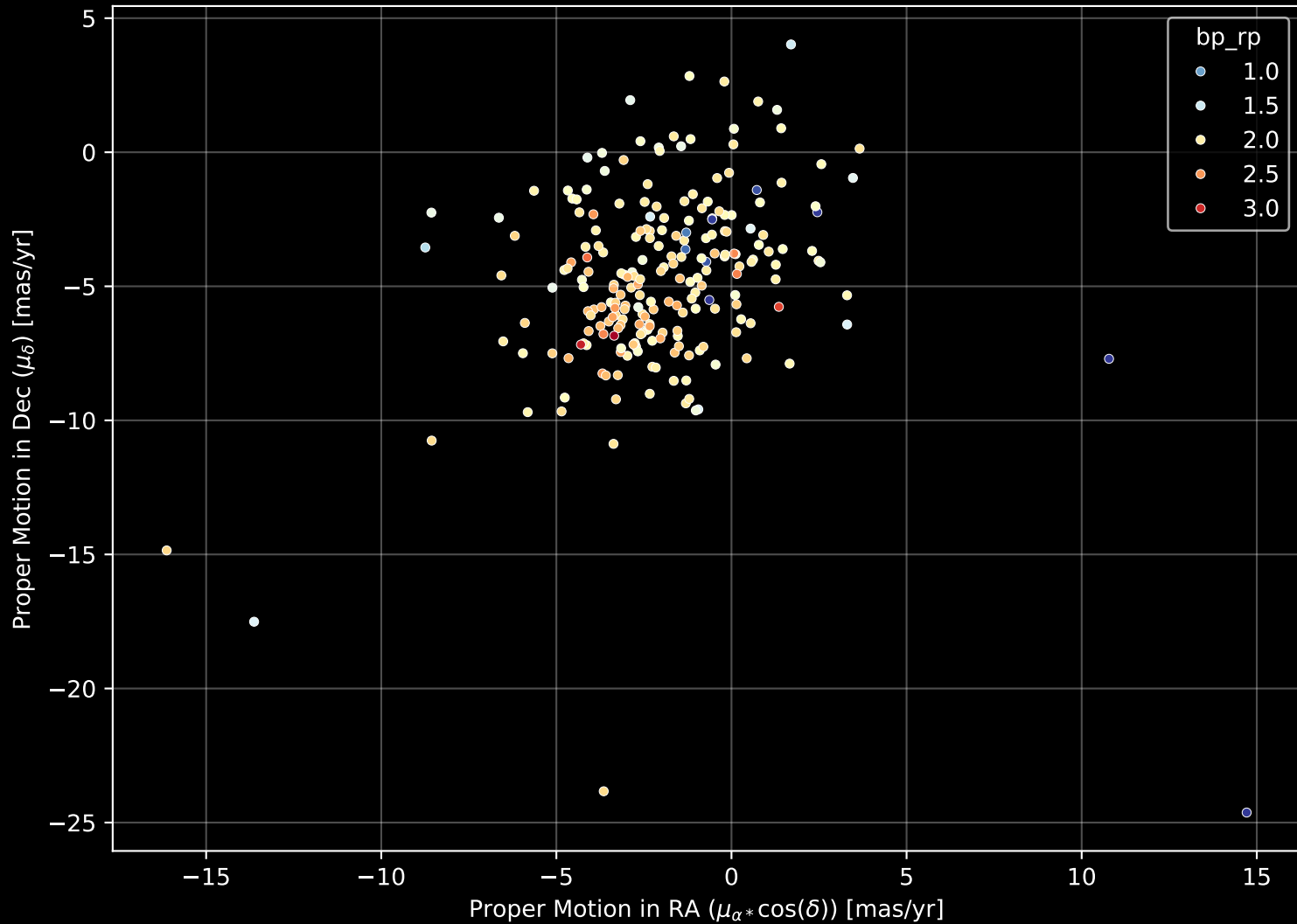
APOGEE DR17 Field: [020-06] Proper Motion Diagram (n= 225)
